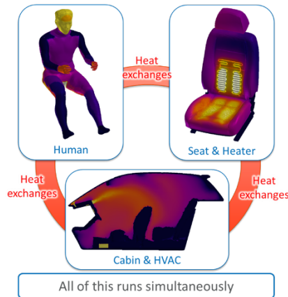
Fig. 8. Coupling Process
